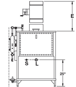
REAR VIEW 4
